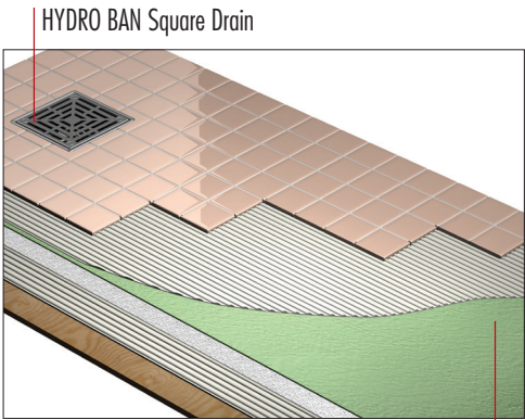
HYDRO BAN Pre-Sloped Shower Pan for Square Drains
